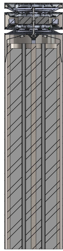
BOLLARD SECTION DETAIL 10-3/4" INNER BOLLARD SECTION VIEW
